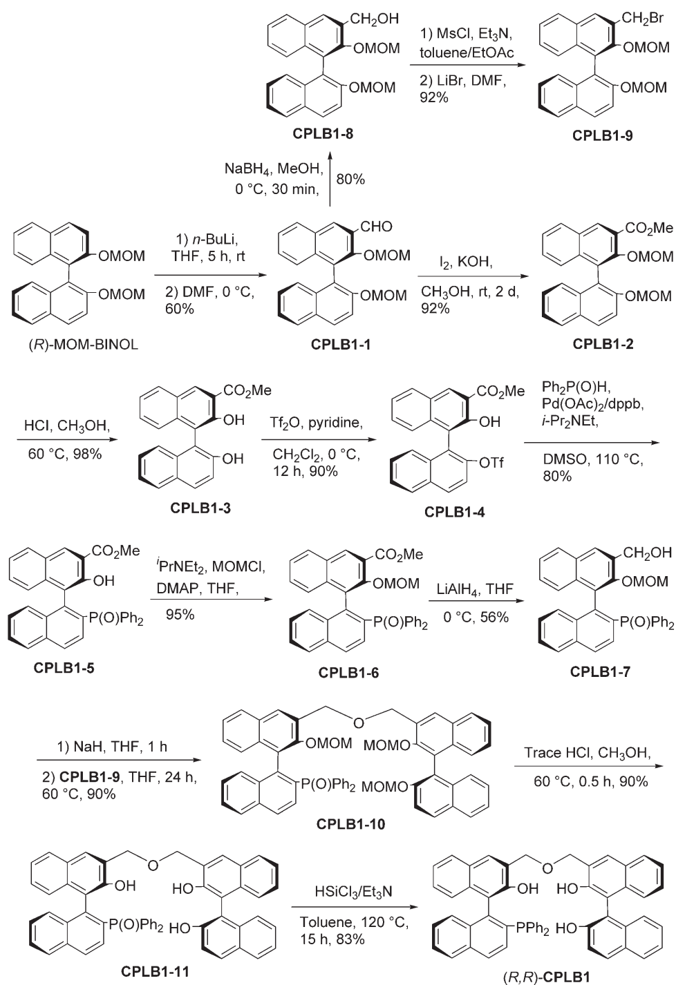
Scheme 1. Synthesis of chiral CPLB1 .
