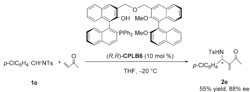
Scheme 3. Asymmetric aza-MBH reaction of N -tosylated aldimine 1e with MVK catalyzed by CPLB6 (10 mol %).
