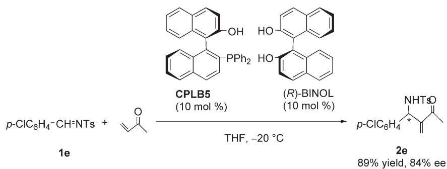
Scheme 4. Asymmetric aza-MBH reaction of N -tosylated aldimine 1e with MVK catalyzed by CPLB5 (10 mol %) and ( R )-BINOL (10 mol %), respectively.
