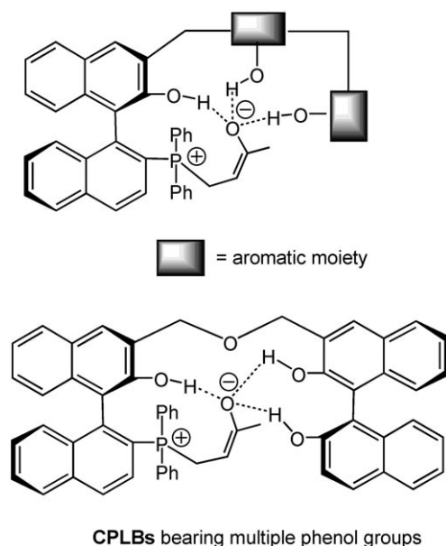
Figure 1. A plausible hydrogen bonding structure in chiral phosphine Lewis bases bearing multiple phenol groups.
