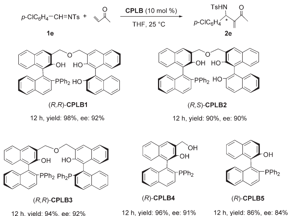
Scheme 2. Asymmetric aza-MBH reaction with chiral phosphine Lewis bases bearing multi-phenolic hydroxy groups in THF at 25 °C.
